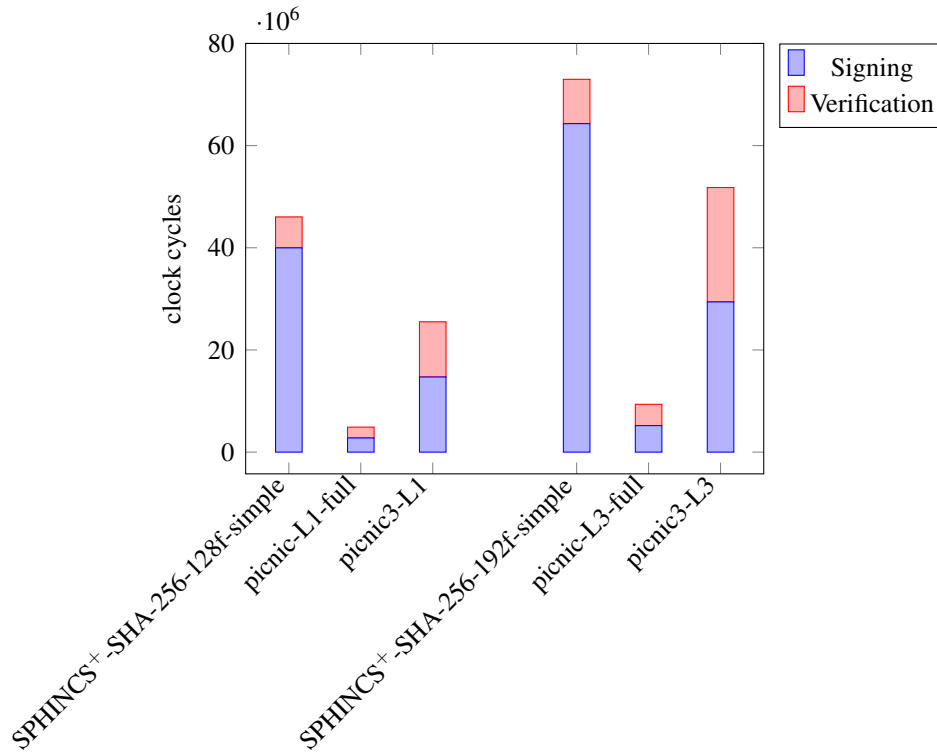
Figure C.1. Picnic and SPHINCS+ Benchmarks on x86_64 processor (using average signature sizes)
