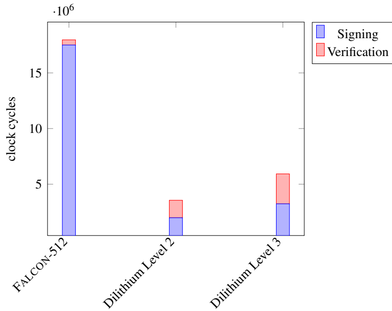
Figure 2.7. Signature Benchmarks on ARM Cortex-M4 processor
