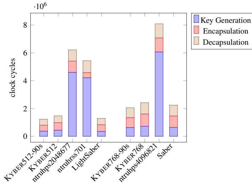
Figure 2.3. KEM Benchmarks on ARM Cortex-M4 processor
