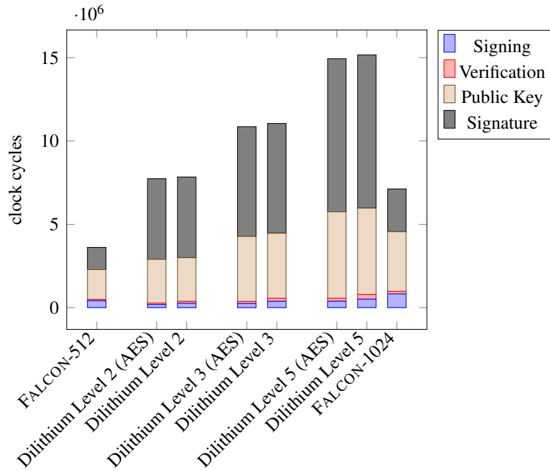
Figure 2.6. Signature Benchmarks on AVX2 processor with 2000 cycles/byte transmission costs
