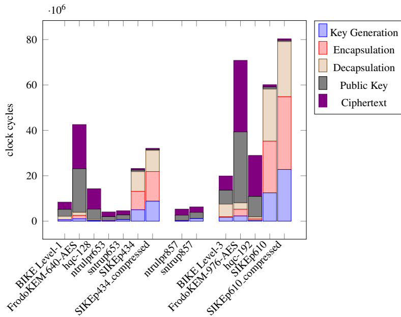
Figure 2.10. KEM Alternates Benchmarks on x86_64 processor with 2000 cycles/byte transmission costs
