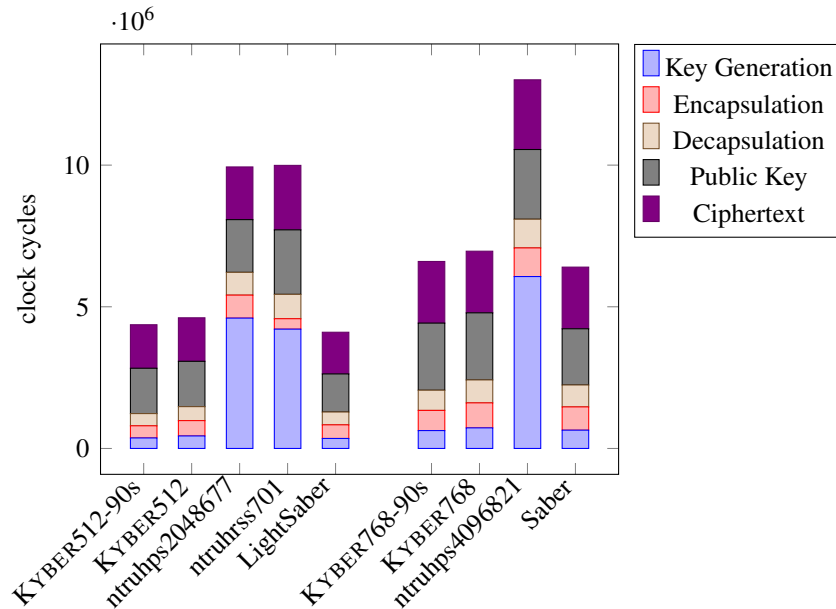
Figure 2.4. KEM Benchmarks on ARM Cortex-M4 processor with 2000 cycles/byte transmission costs
