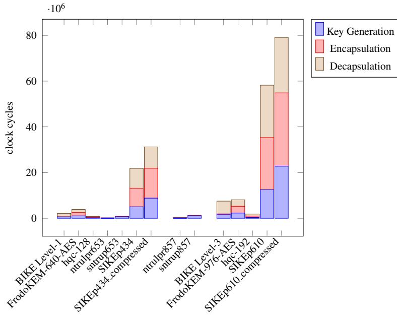
Figure 2.9. KEM Alternates Benchmarks on x86_64 processor
