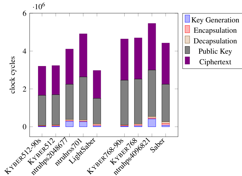
Figure 2.2. KEM Benchmarks on AVX2 processor with 2000 cycles/byte transmission costs
