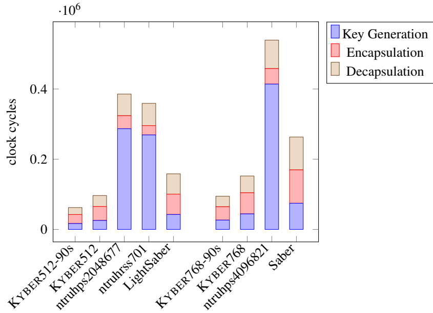
Figure 2.1. KEM Benchmarks on AVX2 processor
