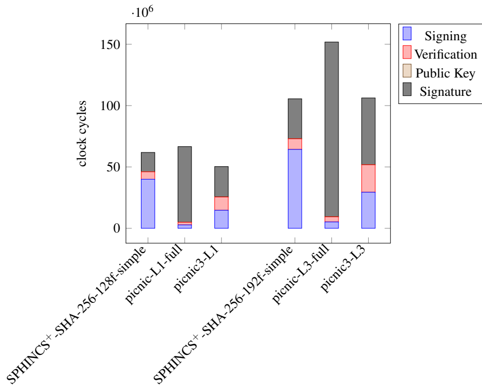
Figure C.2. Picnic and SPHINCS + Benchmarks on x86_64 processor (using average signature sizes) with 2000 cycles/byte transmission costs
