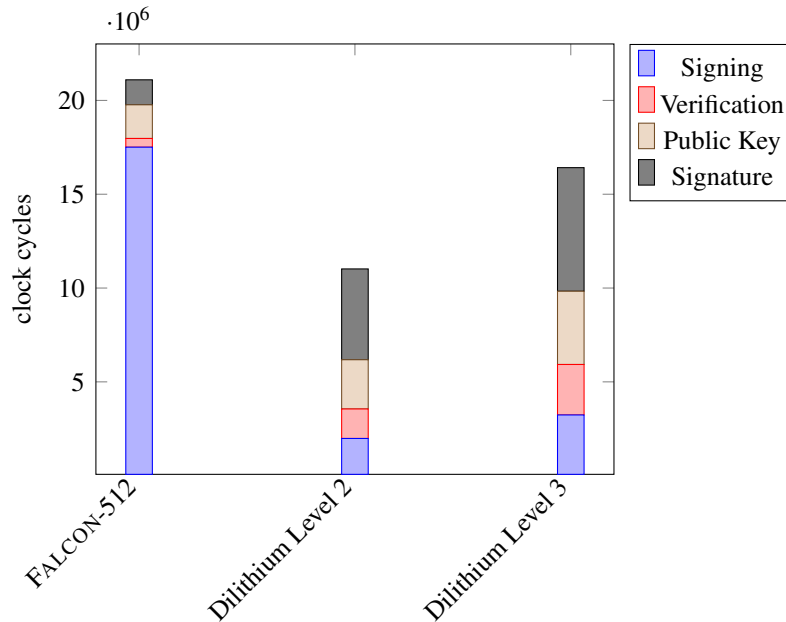
Figure 2.8. Signature Benchmarks on ARM Cortex-M4 processor with 2000 cycles/byte transmission costs
