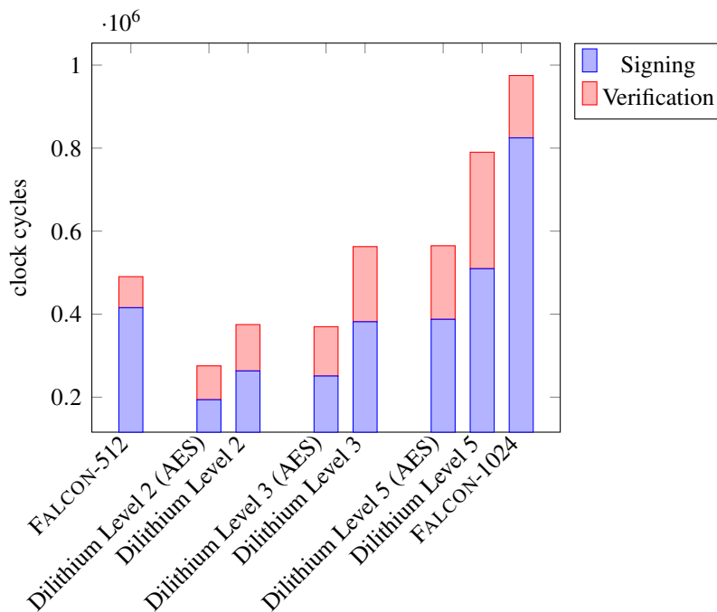
Figure 2.5. Signature Benchmarks on AVX2 processor
